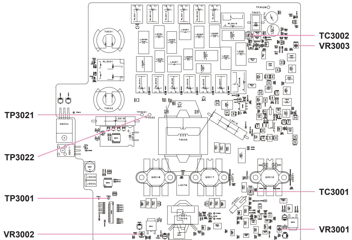
PA Unit (Lot. 1 ~ 68) Alignment Points
