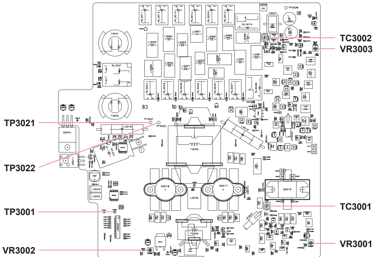
PA Unit (Lot. 69 ~) Alignment Points
