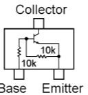
DTC114EU (24) (Q4003, 4006)
