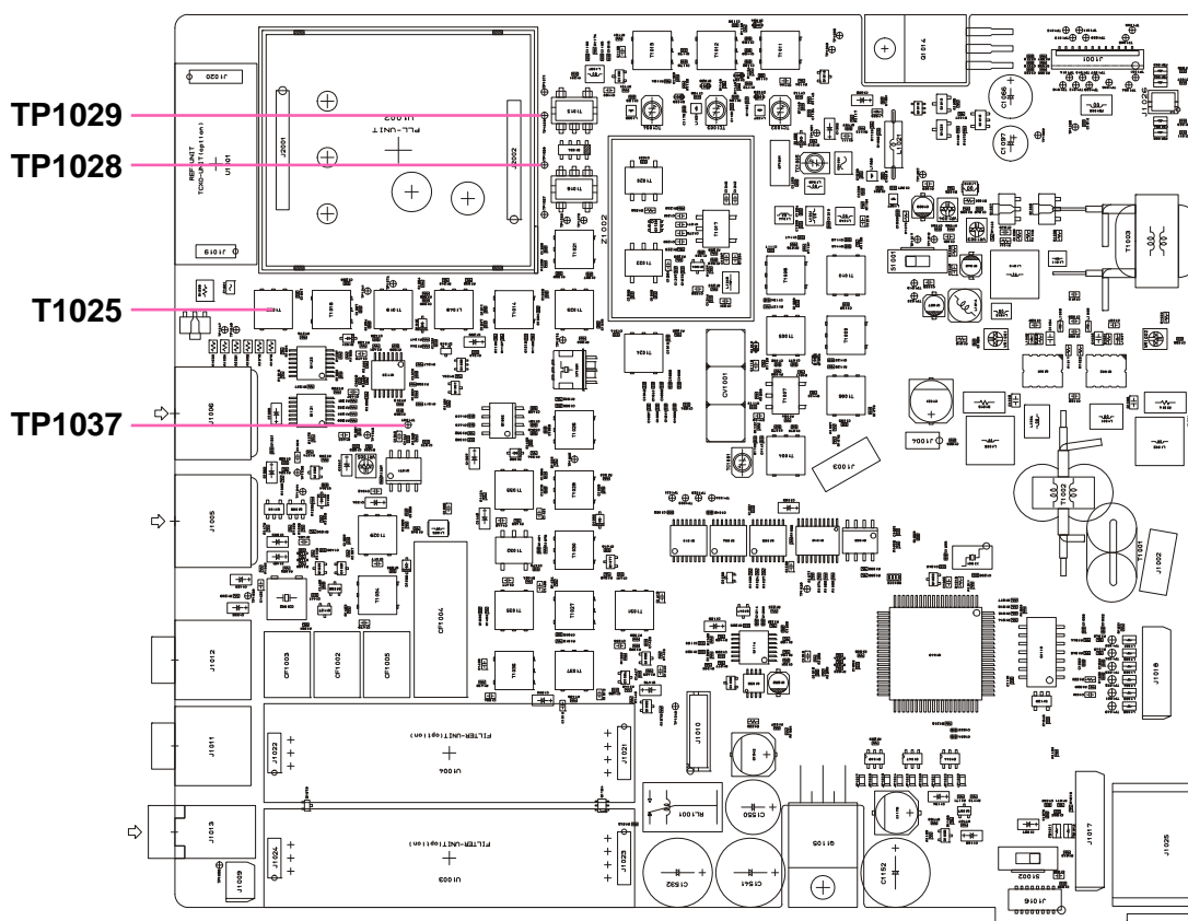
MAIN Unit Alignment Points I
