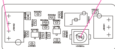
REF Unit Alignment Points
