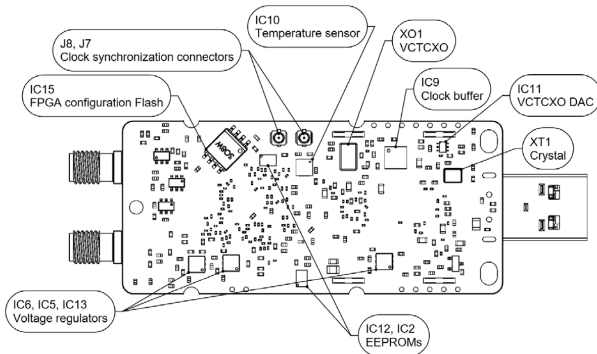
Figure 5: LimeSDR Mini v2.2 board bottom connectors and main components
