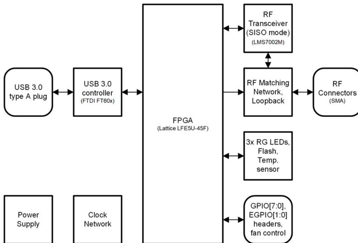
Figure 3: LimeSDR Mini v2.2 Development Board Block Diagram
