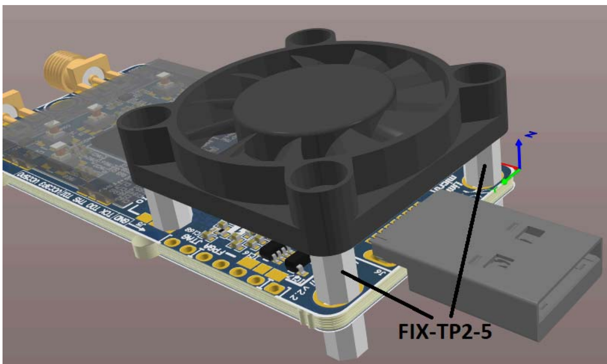
Figure 15: FIX-TP2-5 fan mounting components
