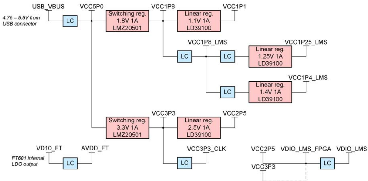
Figure 12: LimeSDR Mini v2.2 board power distribution block diagram
