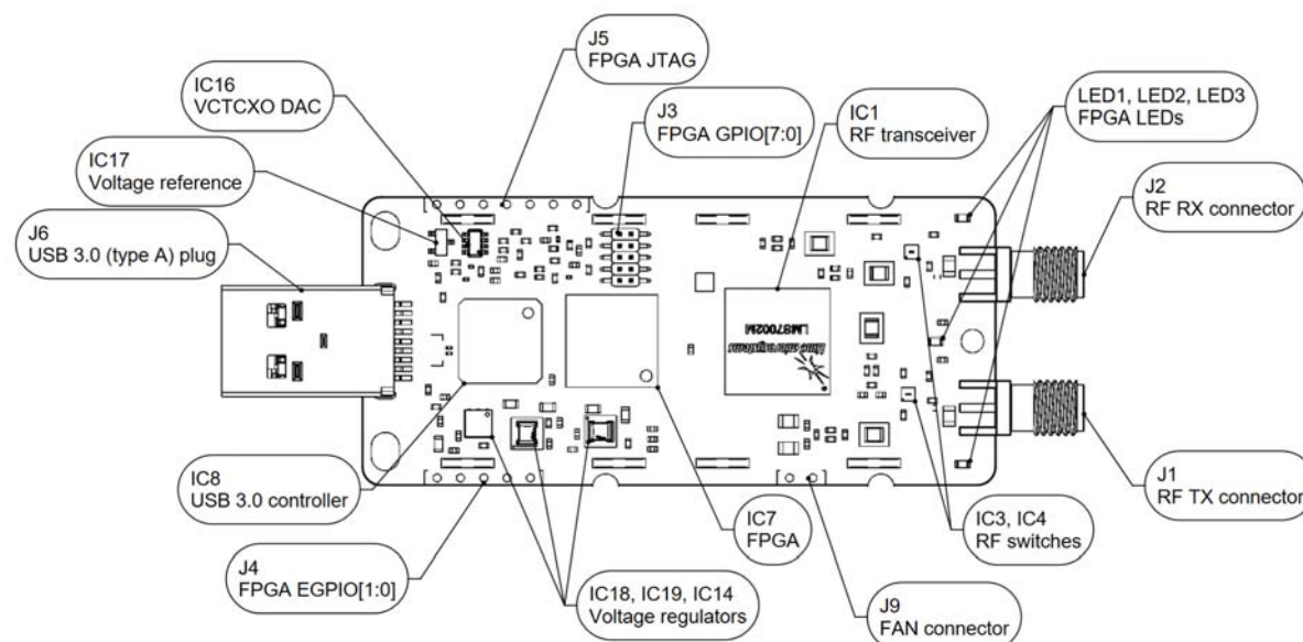
Figure 4: LimeSDR Mini v2.2 board top connectors and main components
