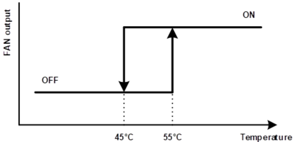
Figure 10: FAN control temperature hysteresis
