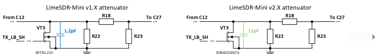
Figure 7: LimeSDR Mini RF loopback attenuator implementation on v1.x and v2.x boards
