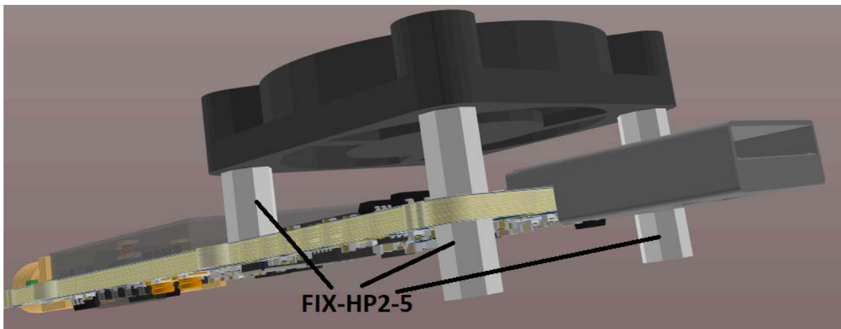
Figure 16: FIX-HP2-5 fan mounting components
