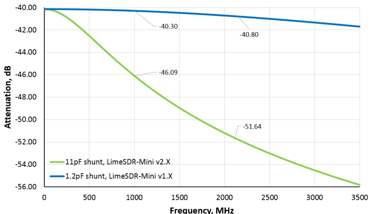
Figure 8: LimeSDR Mini v2.2 RF loopback frequency response
