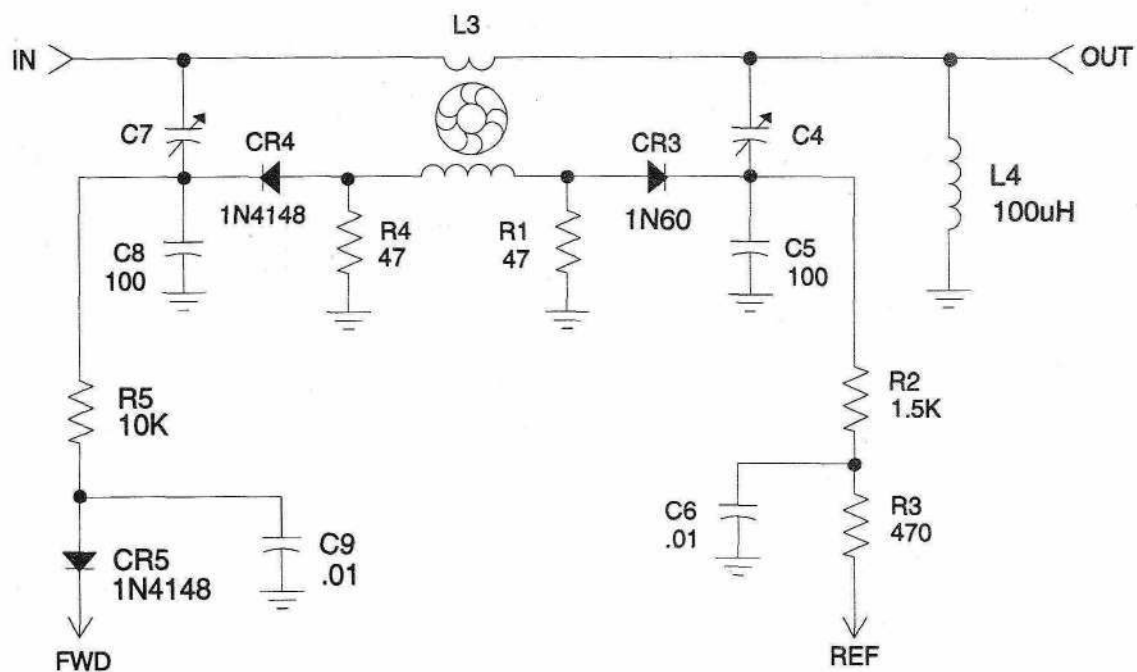
FIGURE 7-SCHEMATIC DIAGRAM, SWR BRIDGE
