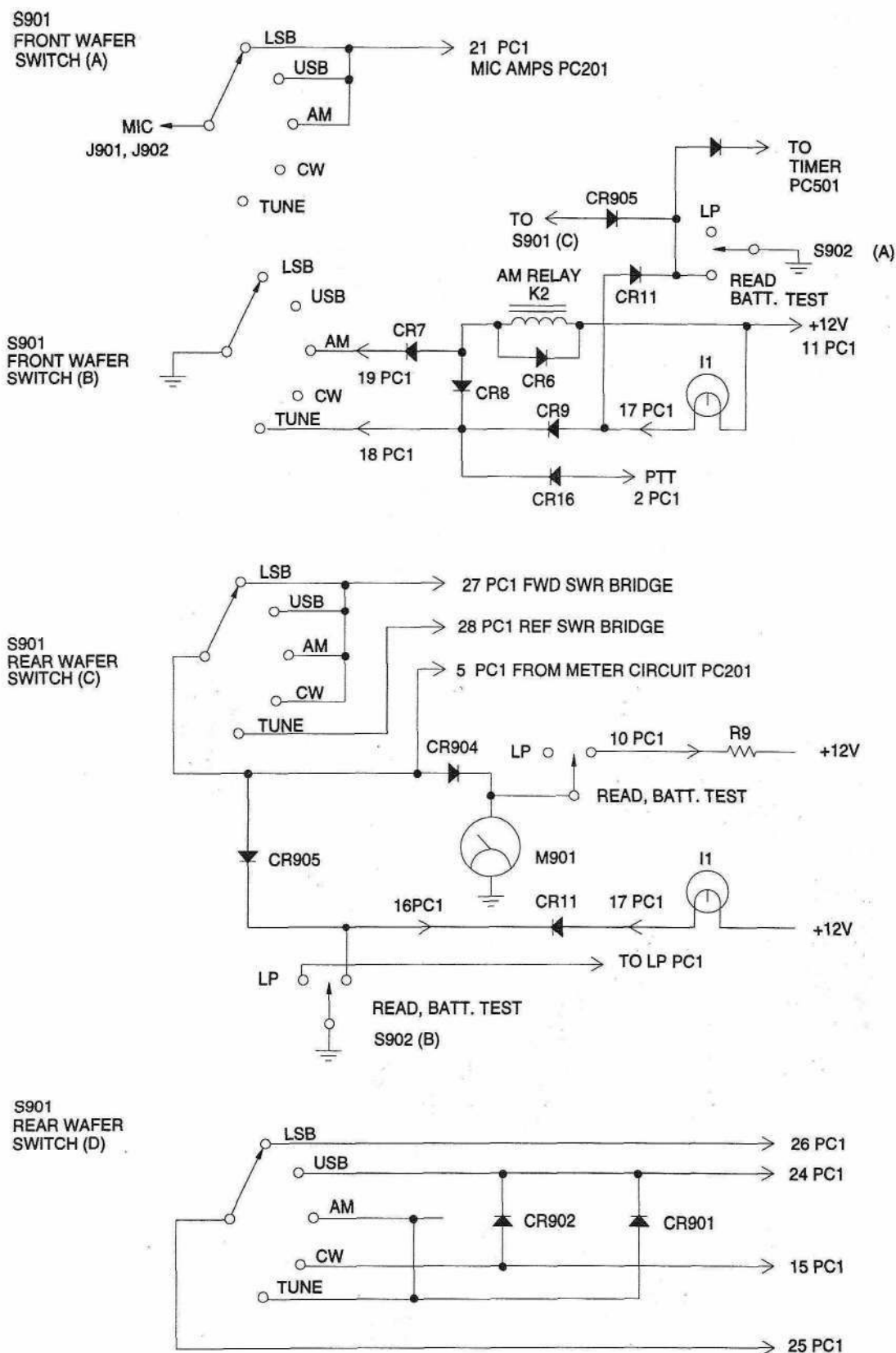
FIGURE 19-SCHEMATIC DIAGRAM, S901/S902 SIMPLIFIED SWITCH CONNECTIONS
