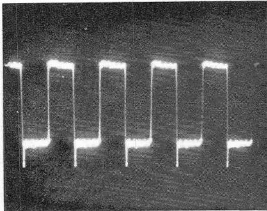
Figure 46 PC501, test point 4, frequency 7 MHz. 1 V per cm. 2 \mu s per division.
