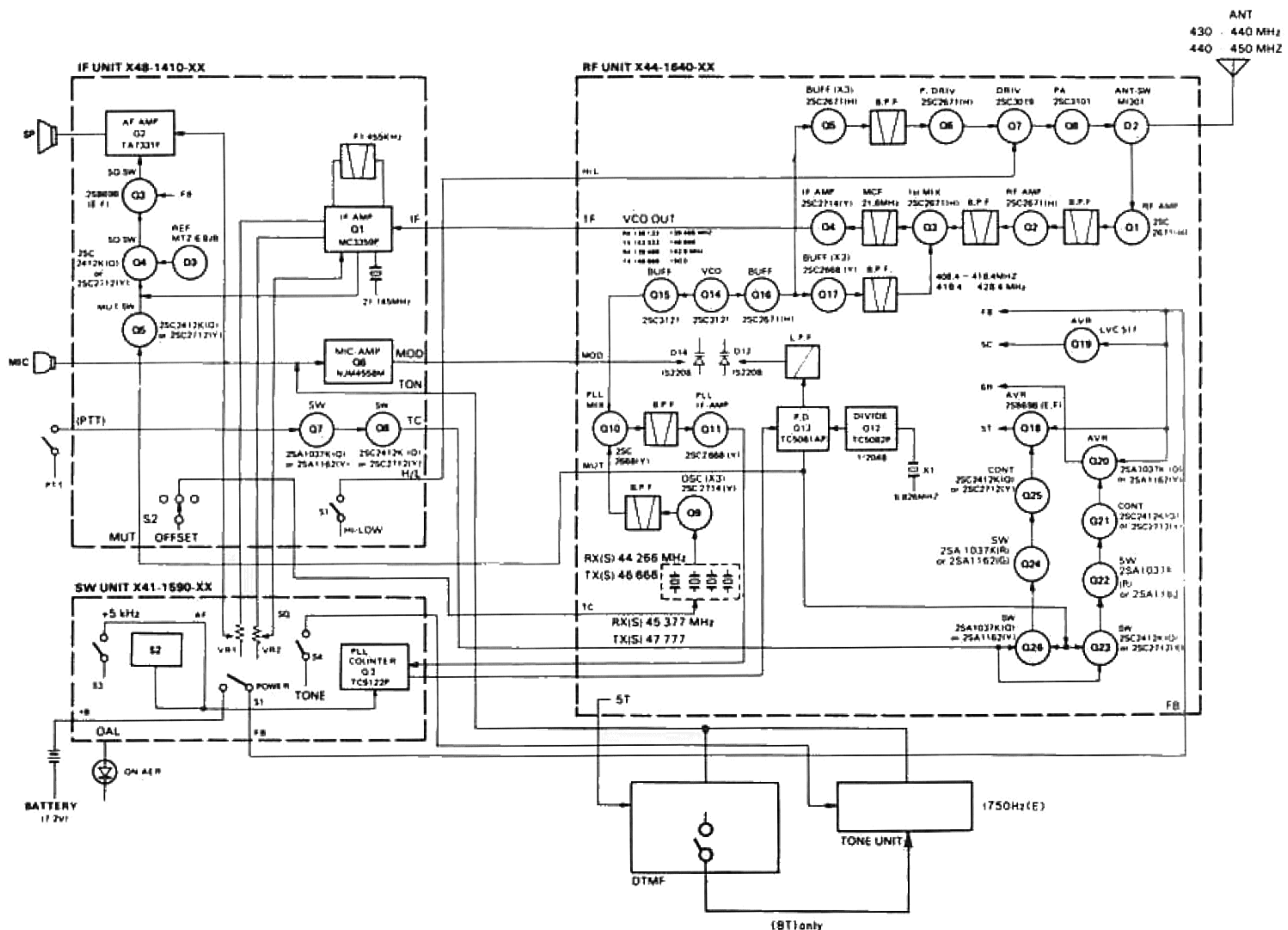
(1) Block Diagram(TH-41A/41BT/41E)
