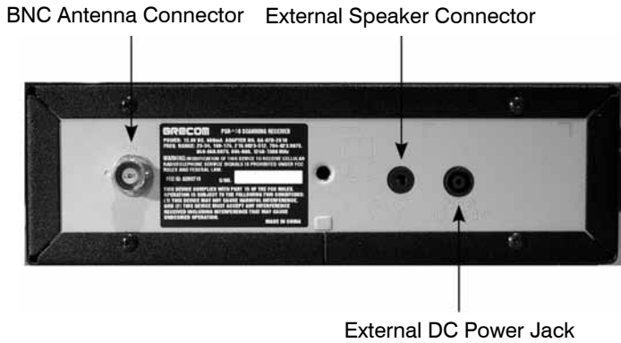
Figure 2 - PSR-410 rear view
