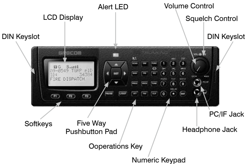
Figure 1 - PSR-410 front view
