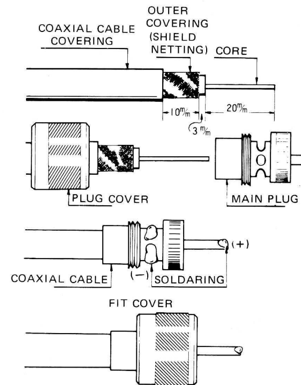
Soldering M-type plug
