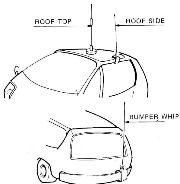
An example of antenna mounting
