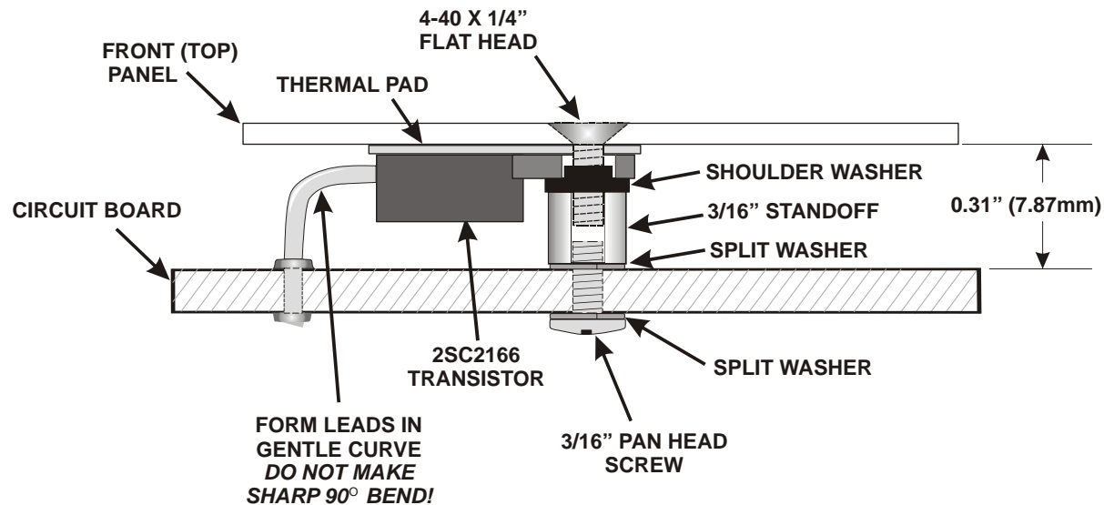
Figure 24. Installing Power Amplifier Q6.
