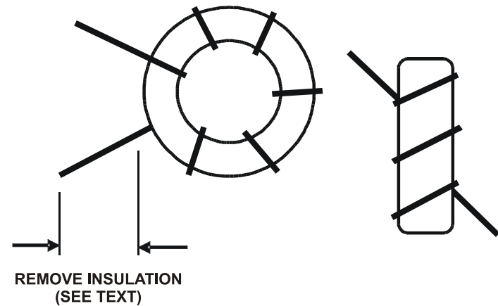
Figure 18. Winding Inductor L3.
