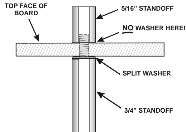
Figure 20. Installing Standoffs on Circuit Board.
