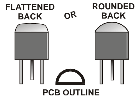
Figure 10. Transistor Orientation Guide.
