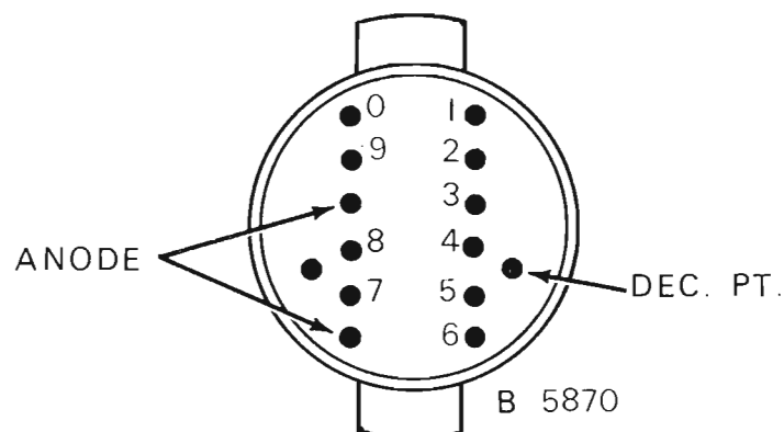
Figure 5-36. Transistor and Readout Indicator Lead Identification
