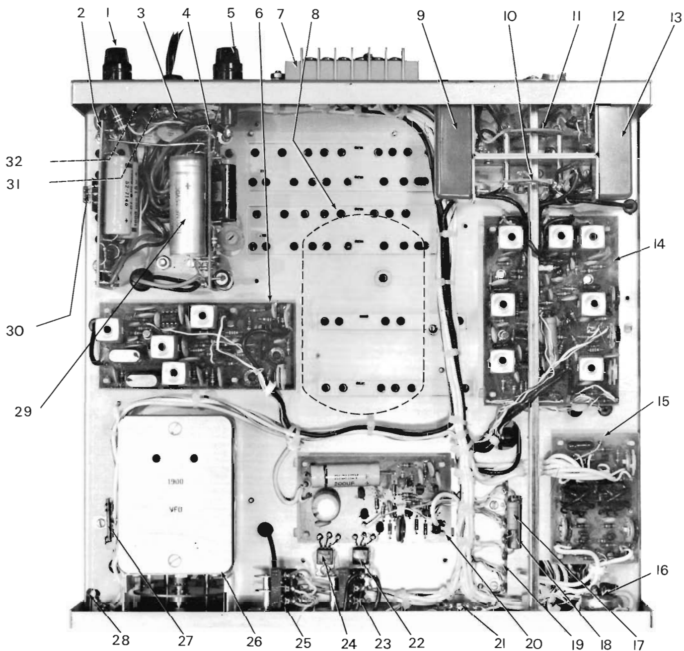
Figure 5-8. Component Locations, Bottom View
