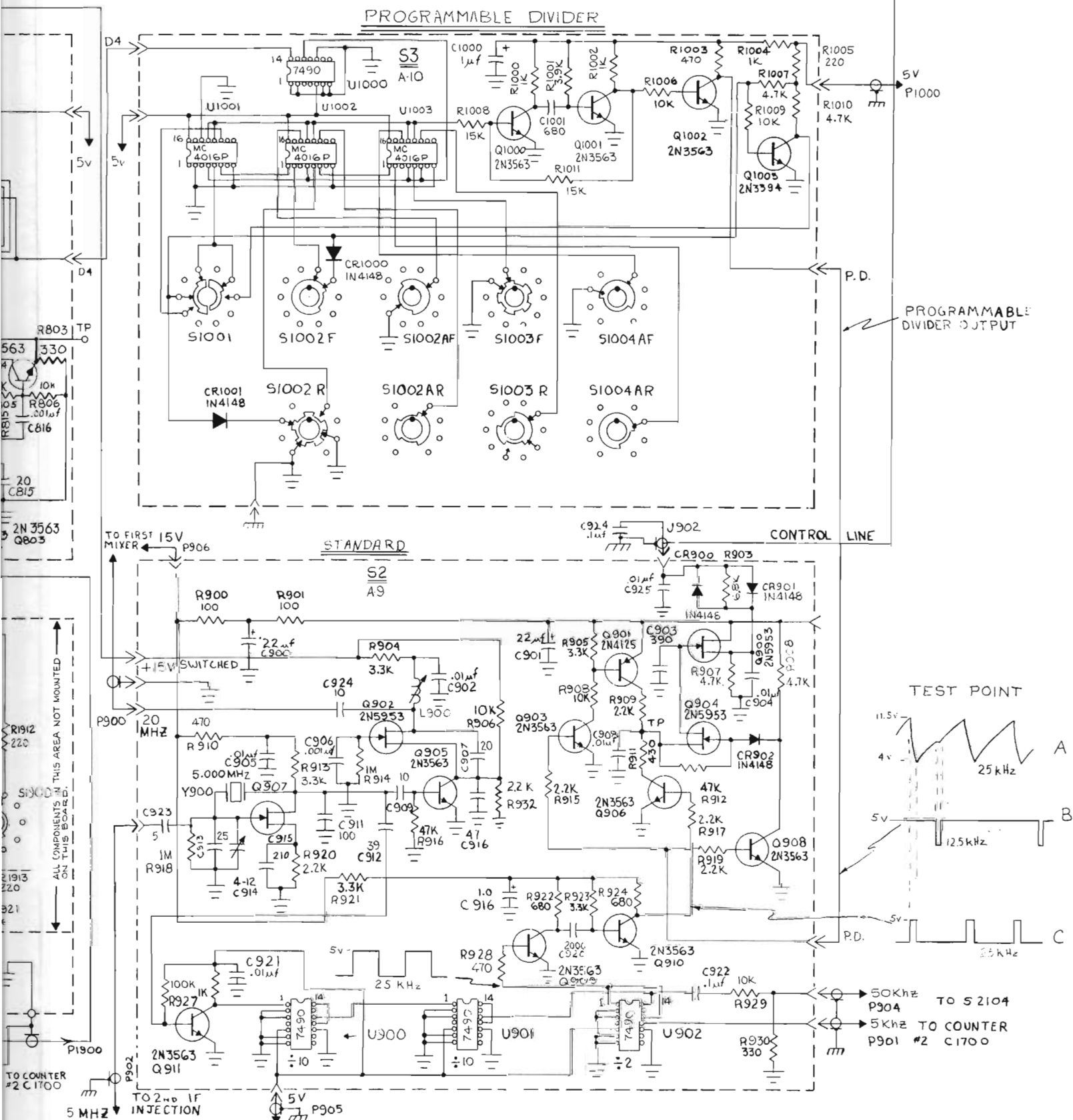
Figure 5–33. Synthesizer, VFO and VCO Schematic
