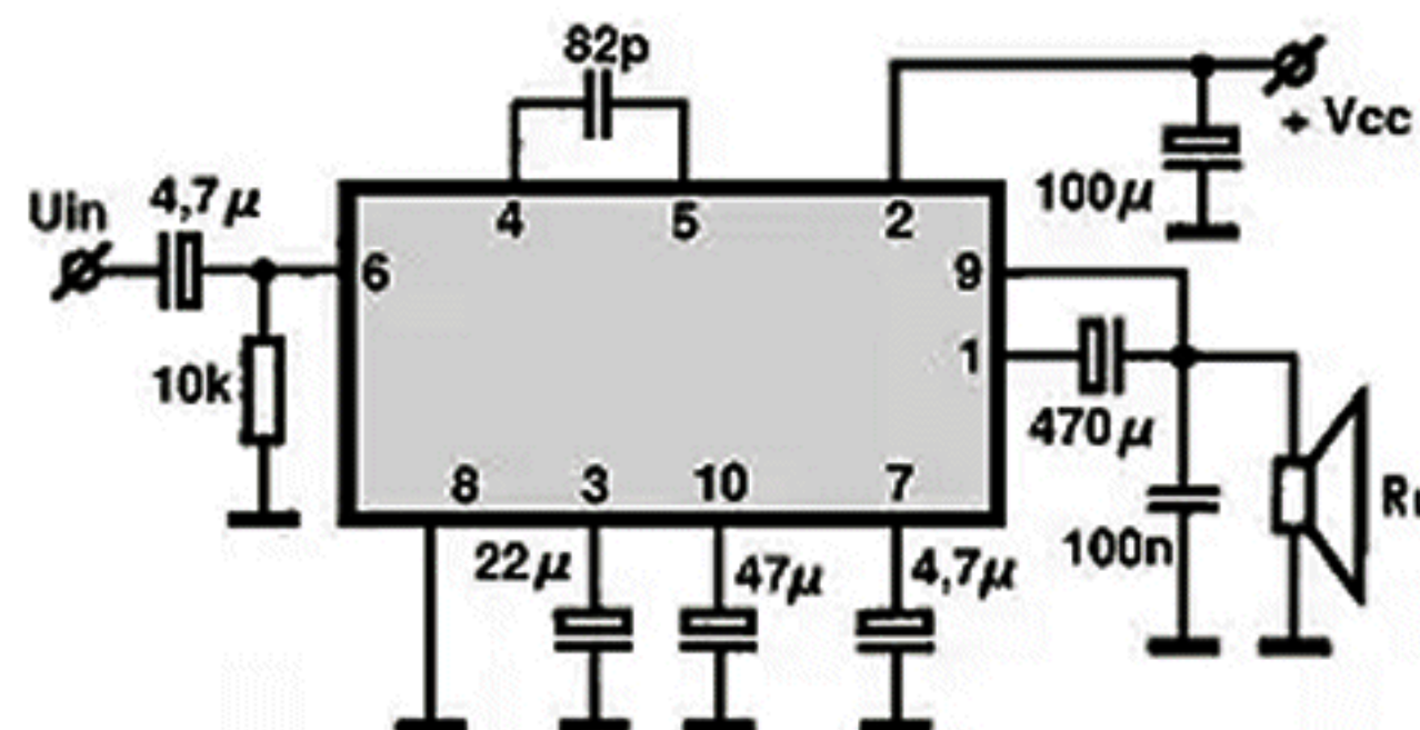
Test circuit
