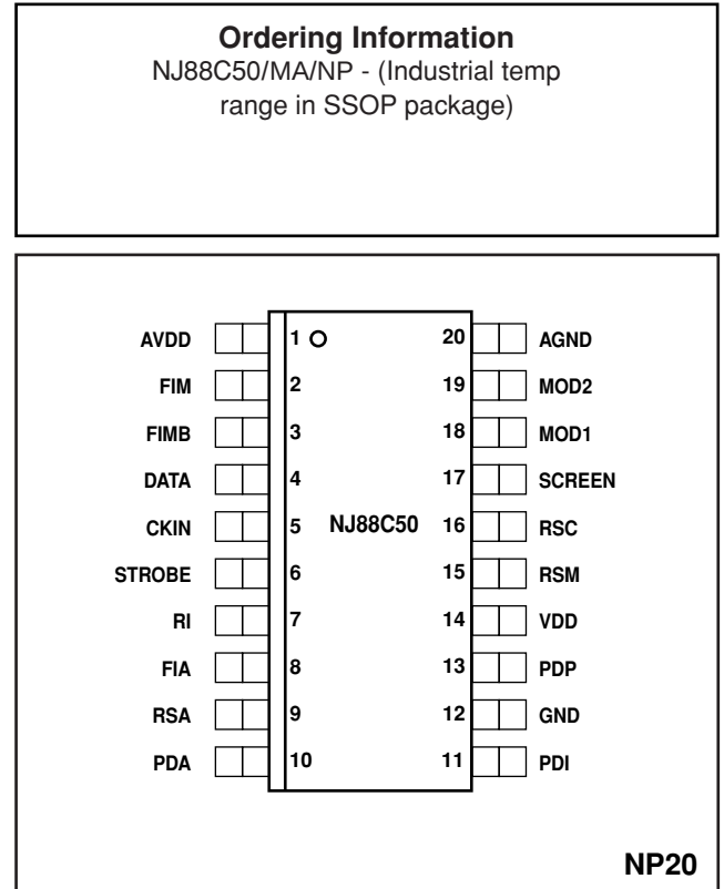
Figure 1 - Pin assignment
