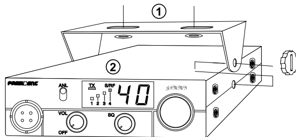
MOUNTING DIAGRAM
