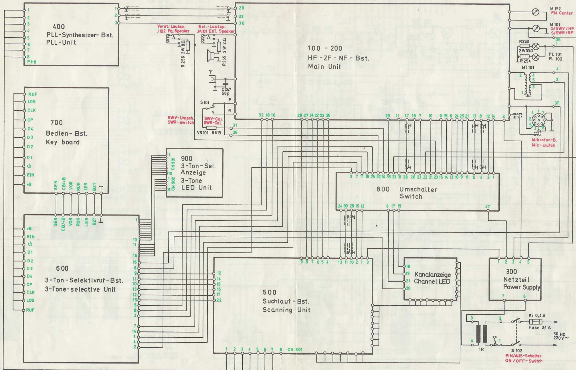
BLOCKSCHALTBIKD BLOCK DIAGRAM
