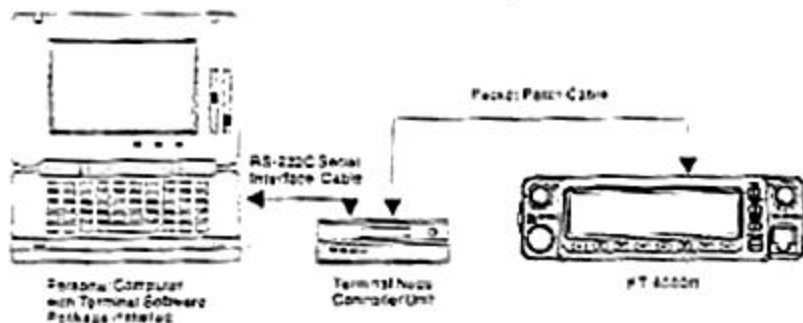
Station Interconnections for Digital Modes
